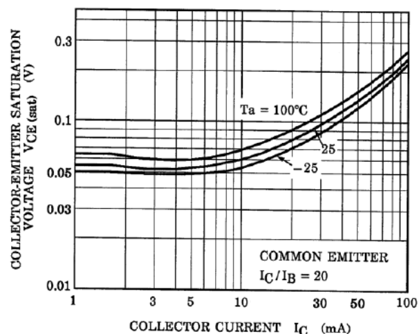
Fig. 10.24 RN1306 V_{CE(sat)}-I_C
