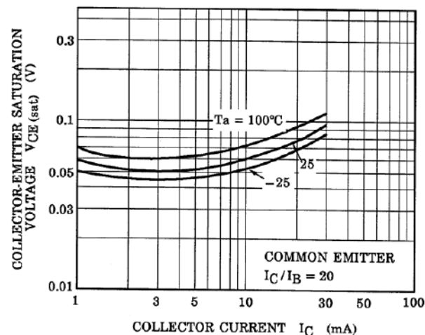
Fig. 10.22 RN1304 V_{CE(sat)}-I_C
