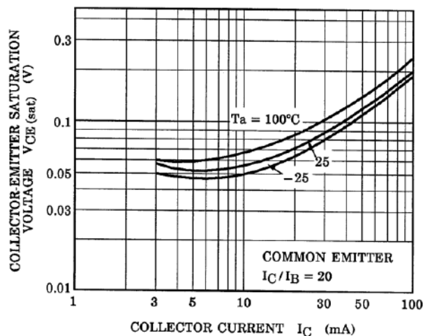
Fig. 10.20 RN1302 V_{CE(sat)}-I_C
